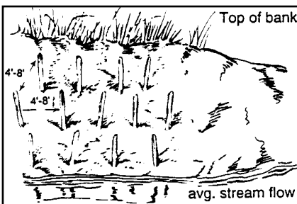
Figure 3. Post spacing on stream bank.
