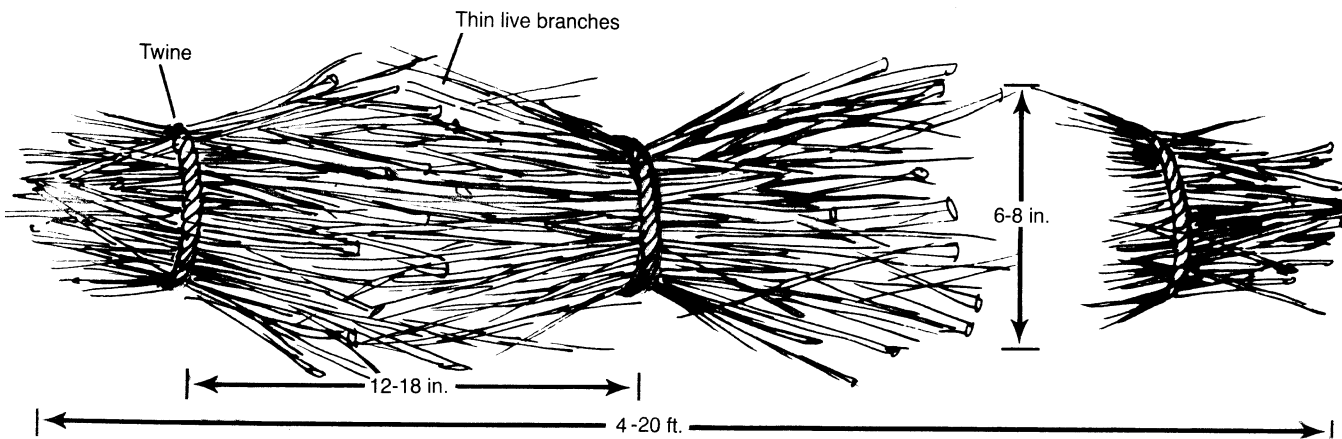
Figure 3. Fascine bundle
