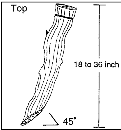
Figure 2. Stake size and shape.
