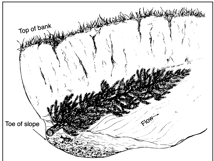
Figure 1. Evergreen Revetment
