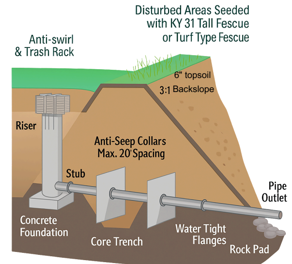
Typical Dam Cross-section
