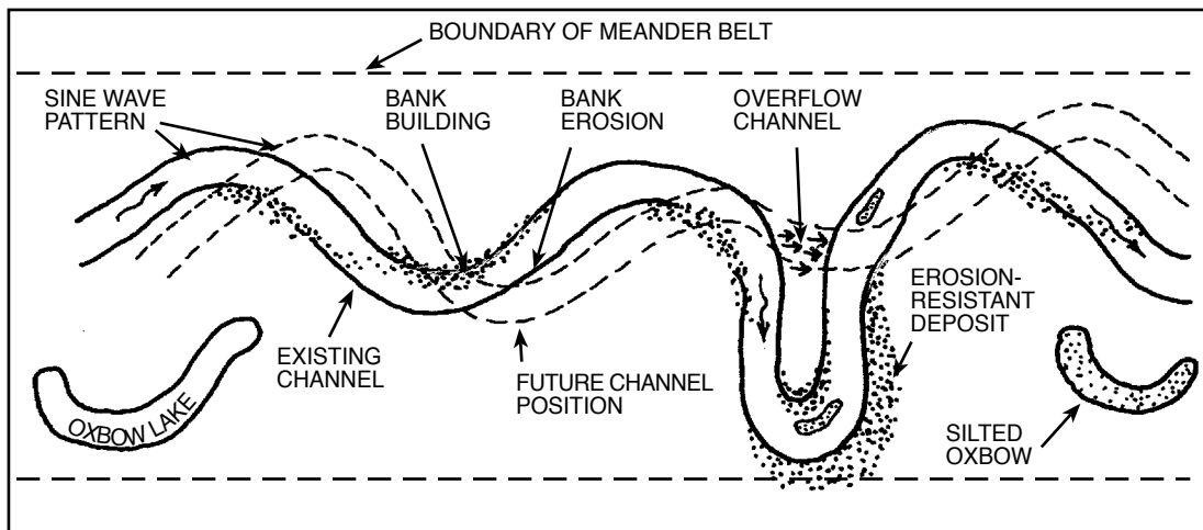
Figure 4. Meandering Stream in an Alluvial Floodplain
